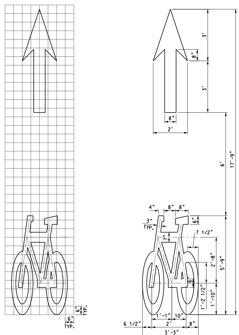
BIKE LANE SYMBOL DETAIL
